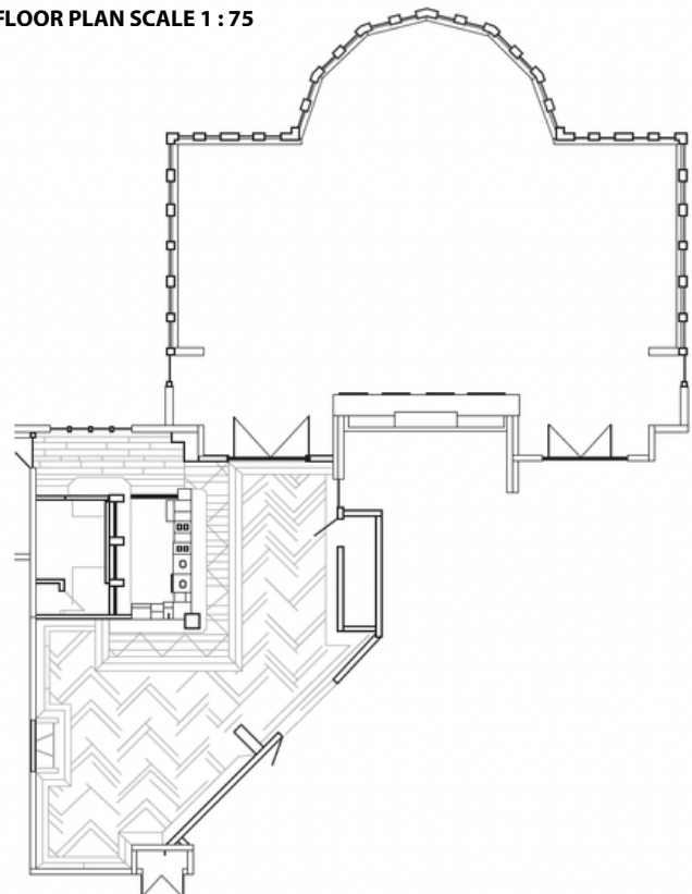
FLOOR PLAN SCALE 1 : 75
